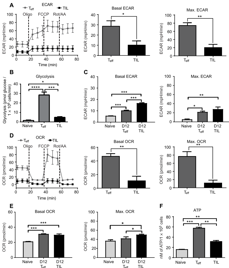
Fig. 1. CD8 + TILs are metabolically less active than acute T eff , but more active than quiescent CD8 + T cells. (A to F) Naive and antigen-specific T eff (day 5 and day 12) were FACS-sorted from the spleens of C57Bl/6 mice immunized with OVA protein, poly I:C, and anti-CD40, whereas antigen-experienced CD8 + TILs were FACS-sorted from B16cOVA melanoma tumors that developed subcutaneously in C57Bl/6 mice for 12 to 15 days. (A to C) Ex vivo T cell glycolytic metabolism as measured by the ECAR (A and C) or the amount of tritiated water ([ 3 H]H 2 O) released from [ 3 - 3 H]glucose during glycolysis (B). The basal ECAR was measured in unmanipulated cells, whereas the maximum ECAR was quantified after exposing cells to a mitochondrial ATP synthase inhibitor (1 μM oligomycin) during the extracellular flux assay. (D and E) Oxidative metabolism (OXPHOS) of the cells in (A) and (C) as quantified by OCR. Basal OCR was from sorted cells in the steady state, whereas maximum OCR was from cells in response to exposure to an uncoupler of mitochondrial OXPHOS (1 μM FCCP). (F) Intracellular ATP levels in sorted ex vivo naive CD8 + T cells, day 5 (d5) T eff , and d14 CD8 + TILs as measured by a luciferase-based ATP determination kit. Data in (A), (C), (D), and (E) are representative of at least three independent experiments where samples were sorted from n = 3 to 5 mice per group and then pooled in each experiment. Data used to generate the graph in (B) were compiled from two independent experiments where the indicated sorted T cell samples were pooled from n = 5 to 9 mice per group. Data in (F) are representative of three independent experiments with samples pooled from n = 3 to 5 mice per group in each experiment. Data in (A) and (D) show means \pm SEM and are analyzed by unpaired Student's t test. Data in (B), (C), (E), and (F) show means \pm SEM and analyzed by one-way ANOVA, followed by Tukey's multiple comparison test. * P < 0.05 , ** P < 0.01 , *** P < 0.001 , **** P < 0.0001 .
