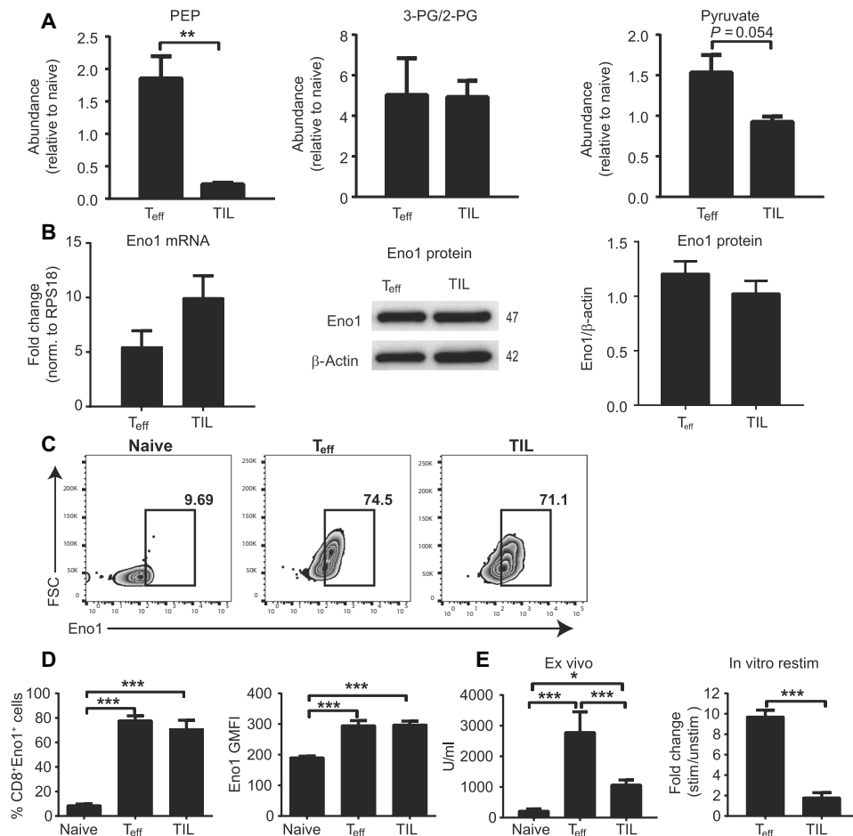
Fig. 4. Weak enolase activity restrains glucose metabolism in glycolysis in CD8 + TILs. (A) Metabolomic analysis of the relative metabolite composition of d5 T eff and d14 CD8 + TILs normalized to that of naive CD8 + T cells. Metabolites were extracted from similar samples to that described in Fig. 1 and subjected to mass spectrometric analysis. 3-PG/2-PG, 3-phosphoglycerate and 2-phosphoglycerate. (B) The expression of enolase 1 transcripts in d5 T eff and d14 CD8 + TILs was measured by qPCR and ENOLASE1 protein was measured by Western blot (numbers indicate molecular weight). (C and D) Flow cytometric analysis of ENOLASE 1 protein expression in naive CD8 T cells, d5 T eff , and d14 CD8 + TILs. The frequencies of cells that express ENOLASE 1 within naive CD8 + CD44lo and OVA-specific CD8 + CD44hi T eff or CD8 + TILs are indicated. GMFI is derived from ENOLASE 1-expressing cells. (E) Fluorescence-based spectrophotometric analysis of enolase activity (PEP formation) measured in lysates prepared from FACS-sorted naive CD8 + T cells, acute T eff , and CD8 + TILs either directly ex vivo (left) or after in vitro stimulation with anti-CD3 and anti-CD28 for 4 days (right). Data are on samples pooled from n = 5 to 9 mice per group (A), representative from two independent experiments with samples pooled from at least six mice per group (B), and are representative of three independent experiments with at least three mice per group (C and D). Data in (E) are combined from multiple independent experiments with T cells pooled from 2 to 3 mice per group. Data show means \pm SEM and are analyzed by unpaired Student's t test (A, B, and E, right) or one-way ANOVA, followed by Tukey's multiple comparison test (D and E, left). * P < 0.05 , ** P < 0.01 , *** P < 0.001 .
