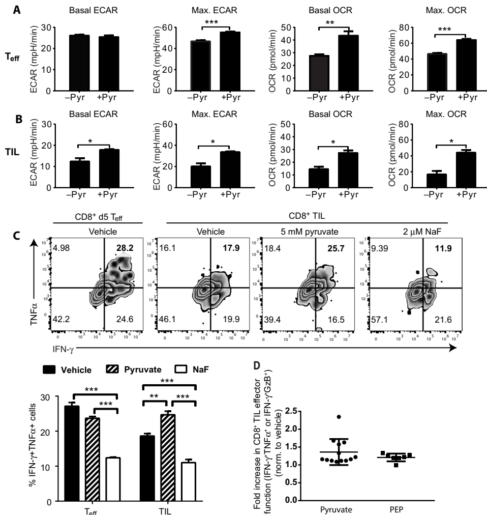
Fig. 5. Bypassing enolase restores metabolic function and effector activity in CD8 + TILs. (A and B) ECAR and OCR by FACS-sorted d5 T eff and d12 CD8 + TILs as measured by Seahorse in pyruvate-free or 2 mM pyruvate-containing XF minimal media. Basal ECAR and basal OCR were measured without any manipulation, whereas maximum ECAR and maximum OCR were determined after oligomycin or FCCP exposure, respectively. (C and D) Intracellular flow cytometric analysis of IFN-γ and TNFα production from T eff and CD8 + TILs treated for 4 hours with vehicle, 5 mM pyruvate, or 2 μM NaF during in vitro culture and stimulation with OVA 257 -pulsed antigen-presenting cells. (D) Fold increase in the proportion of CD8 + T cells expressing cytokines after culturing with 5 mM pyruvate or PEP (1 μg/ml; after partial permeabilization) for 4 hours. Data are representative of two to three independent experiments and show means ± SEM. Statistical analyses were done by unpaired Student's t test (A, B, and D) and two-way ANOVA, followed by Tukey's multiple comparison test (C). * P < 0.05, ** P < 0.01, *** P < 0.001.
