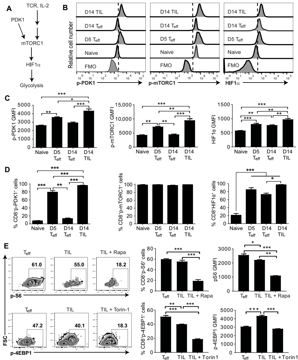
Fig. 3. Glycolysis-regulating signaling molecules are expressed and active in CD8 + TILs. (A) The signaling pathway downstream of TCR and cytokine signals that are known to promote the glucose uptake and glycolysis. (B to D) Flow cytometric analysis of p-PDK1 (Ser 244 ), p-mTORC1 (Ser 2448 ), and HIF1 \alpha expression in naive CD8 + T cells and OVA-specific d5 T eff , d14 T eff , and d14 CD8 + TILs that were prepared as in Fig. 1. (C) GMFI of pPDK1, p-mTORC1, and HIF1 \alpha in the CD8 + CD44lo naive or OVA-specific CD8 + CD44hi T eff and TILs expressing the protein of interest. (D) The frequency of p-PDK1 + , p-mTORC1 + , or HIF1 \alpha + cells within naive CD8 + CD44lo and OVA-specific CD8 + CD44hi T eff and TILs. (E) Phosphoflow cytometric analysis of mTORC1 activity via determination of the phosphorylated downstream targets (S6 and 4E-BP1) after 1-hour in vitro stimulation of acute T eff and CD8 + TILs with anti-CD3 (5 \mu g/ml). The CD8 + TIL in vitro stimulation was also conducted in the presence of 250 \mu M rapamycin to inhibit pS6 or 250 \mu M Torin-1 to inhibit p4E-BP1 for staining negative control. Data in (B) to (D) are representative of three to five independent experiments, with at least two mice per group in each experiment. Data in (E) are from samples pooled from n = 5 to 6 mice per group, and the experiment was repeated twice. Data show means \pm SEM: one-way ANOVA, followed by Tukey's multiple comparison test. * P < 0.05 , ** P < 0.01 , *** P < 0.001 .
